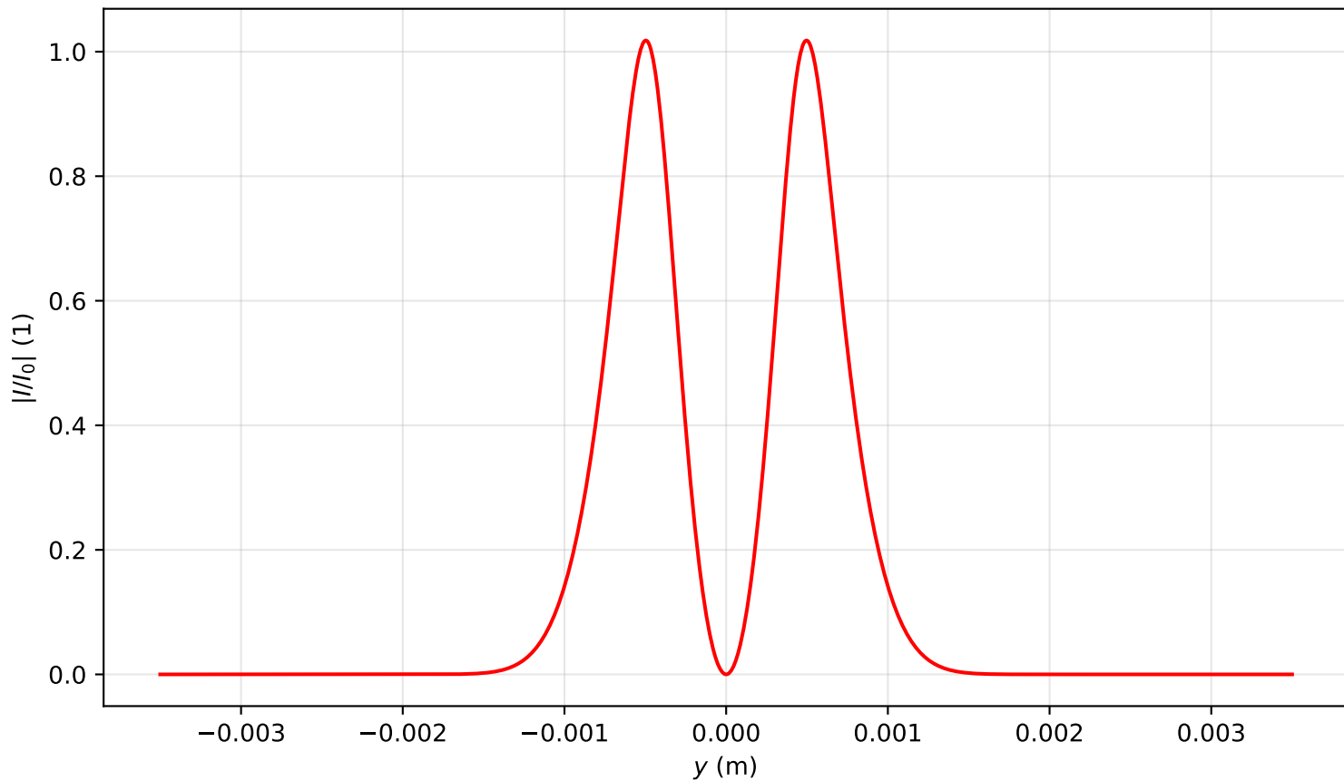
Intensity profile I(x=0, y, z=0.239)/I_0 , P_{in}=6.0P_{cr} , artificial time
